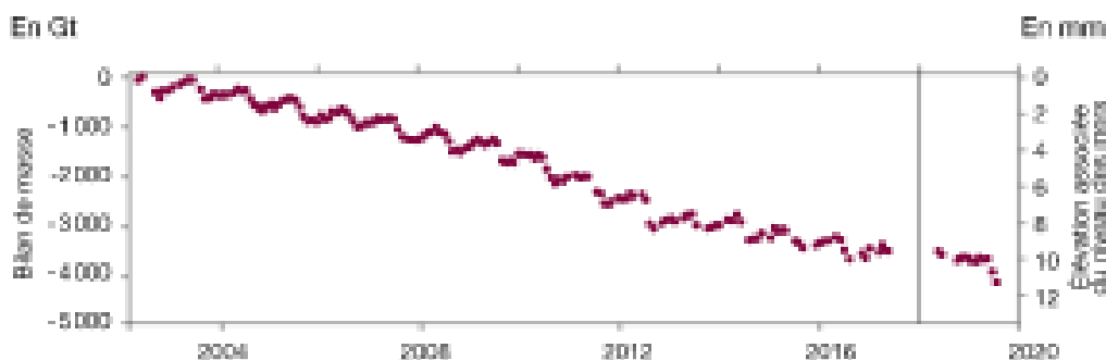
GREENLAND ICE MASS BALANCE FROM 2002 TO 2019
